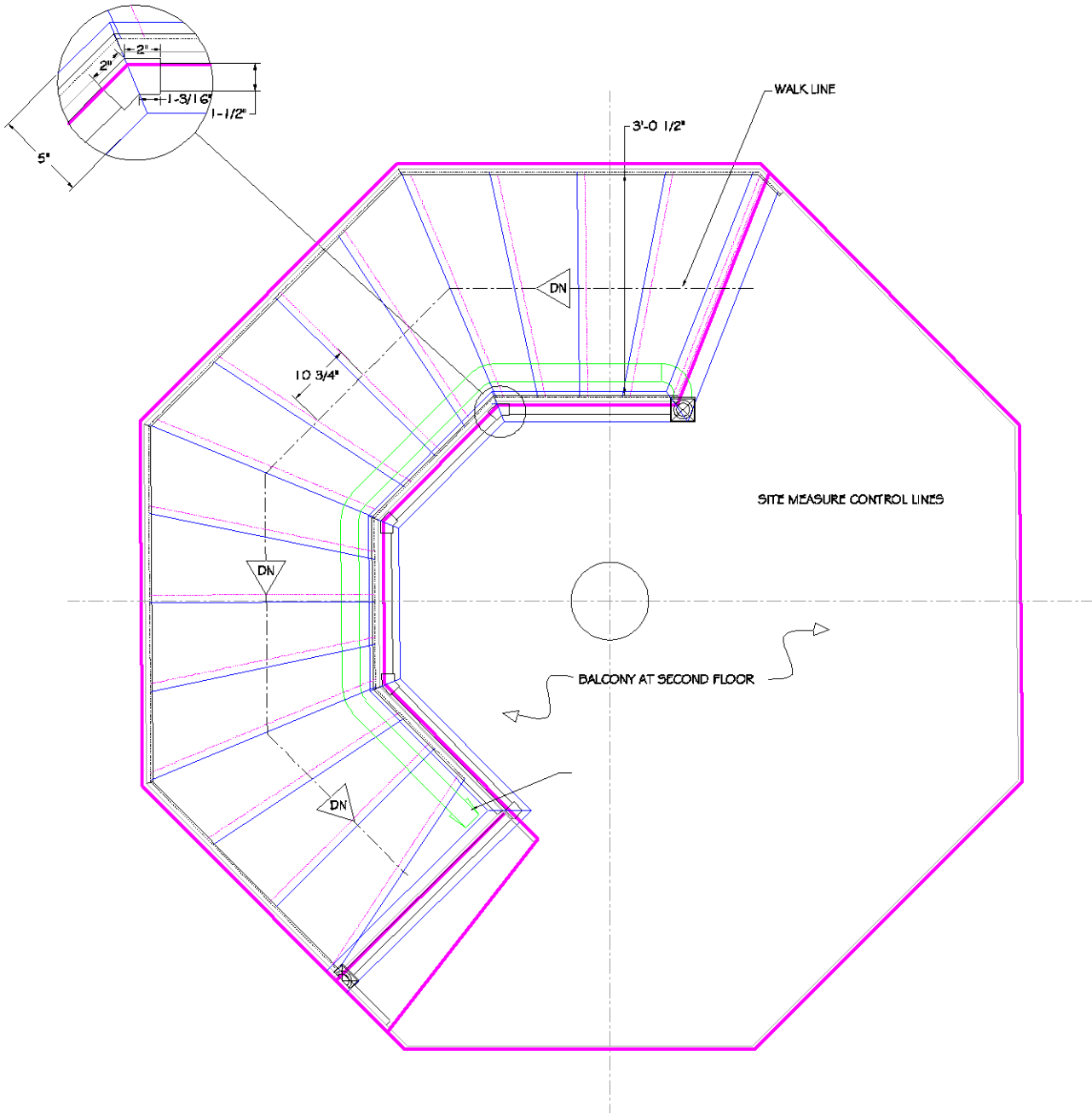
PLAN VIEW OCTAGONAL STAIR FIRST TO SECOND FLOOR
